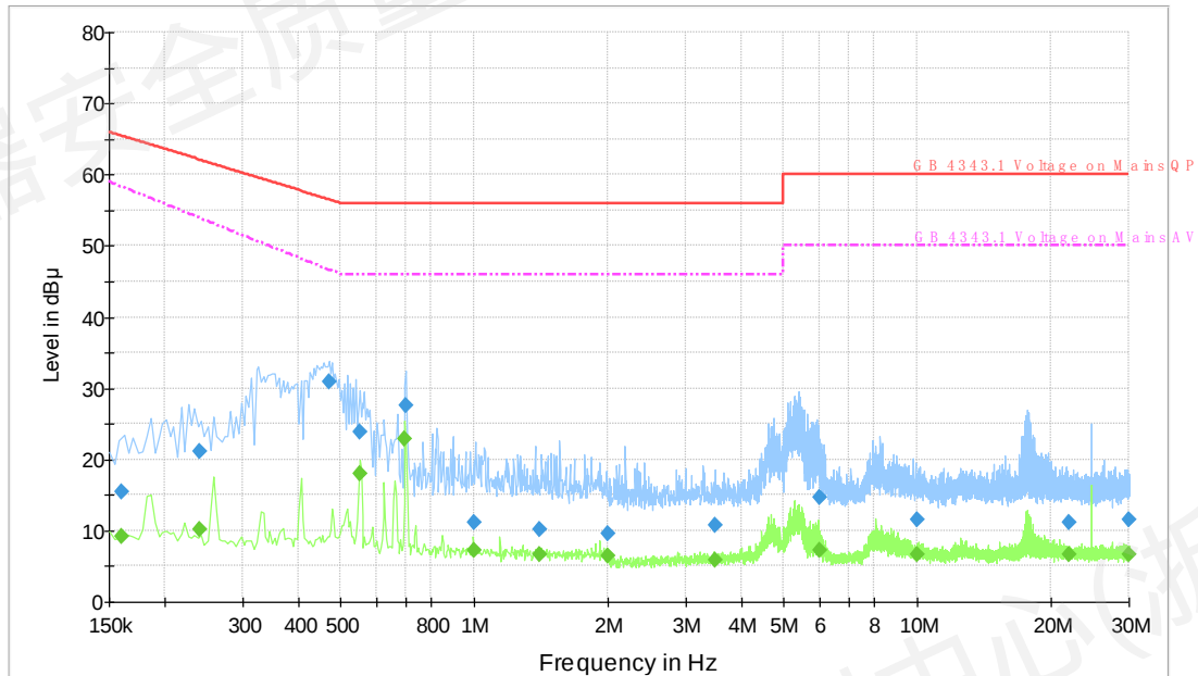
GB 4343.1 Voltage with 4-Line-LISN-2
